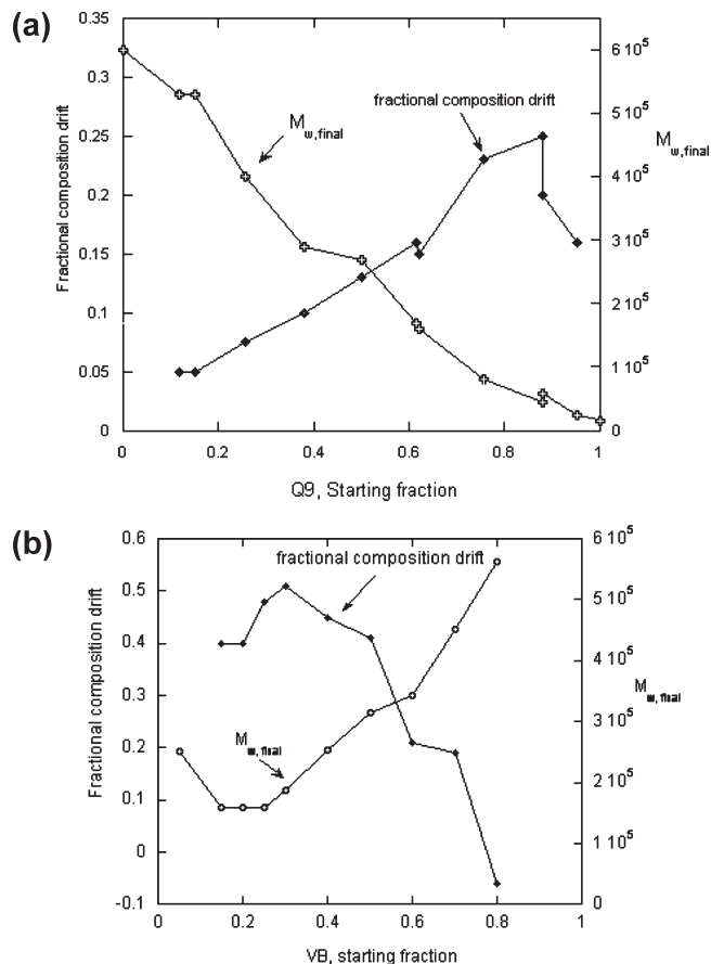
Figure 6. (a) M_{w,final} and total fractional composition drift vs starting fraction of Q9/Am batch reactions ( [Am] + [Q9]/[KPS] = 120 ). (b) M_{w,final} and total fractional composition drift vs starting fraction of VB/Am batch reactions ( [Am] + [VB]/[V50] = 180 ).
